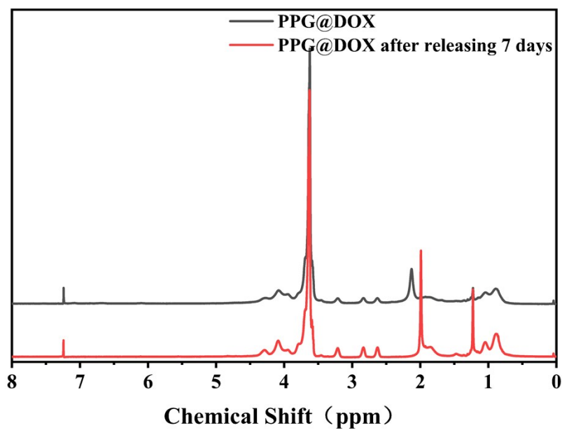
Figure S2. The 1 H-NMR spectra of the materials before and after released for one week.
