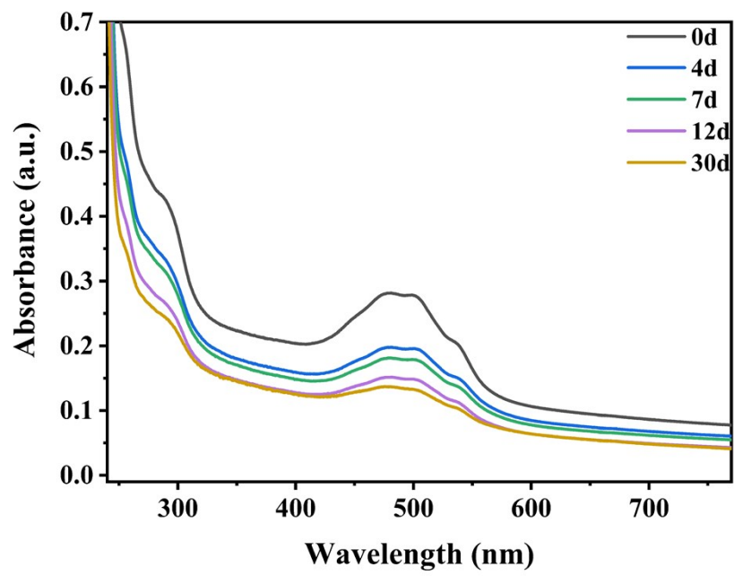
Figure S3. The UV-Vis spectra of the drug release process in buffer solution with pH=5.5.
