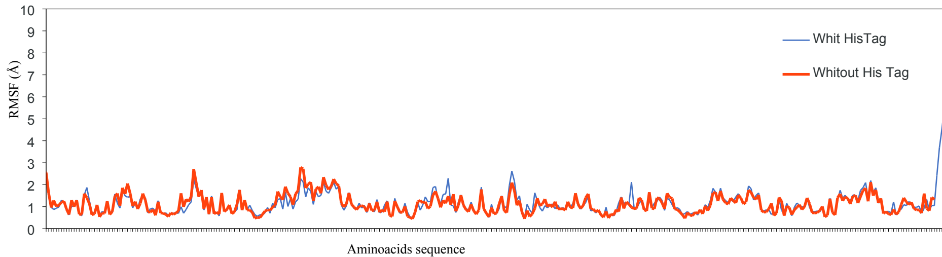
23 Figure 2S. Root-mean-square-fluctuations (RMSF) of the complex BhXyn10AH /ligands obtained by molecular dynamic simulations during 50 ns. Comparison of structures 24 with and without 6x C-histidine tag. Notice that the histidine tag is very flexible.
