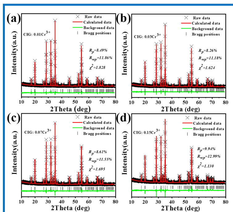
Fig. S2 (a-d) Rietveld refinement X-ray diffraction of \text{CIG}:x\text{Cr}^{3+} ( x = 0.01, 0.03, 0.07, 0.15 ).
