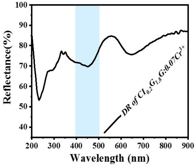
Fig. S3 Diffuse reflectance spectra (DR) of \text{Cl}_{0.2}\text{G}_{1.8}\text{G}:0.07\text{Cr}^{3+} .
