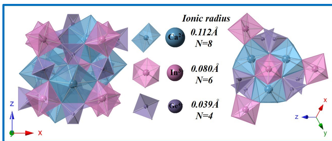
Fig. S1 Crystal structure and ionic oxygen coordination environment of \text{Ca}_3\text{In}_2\text{Ge}_3\text{O}_{12} .
