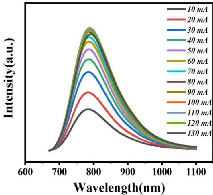
Fig. S4 Emission spectra of the \text{Cl}_{0.2}\text{G}_{1.8}\text{G}:0.07\text{Cr}^{3+} pc-LED under various drive currents.
