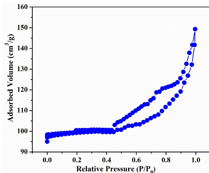
Figure S1. BET analysis for NMc-CuTA
