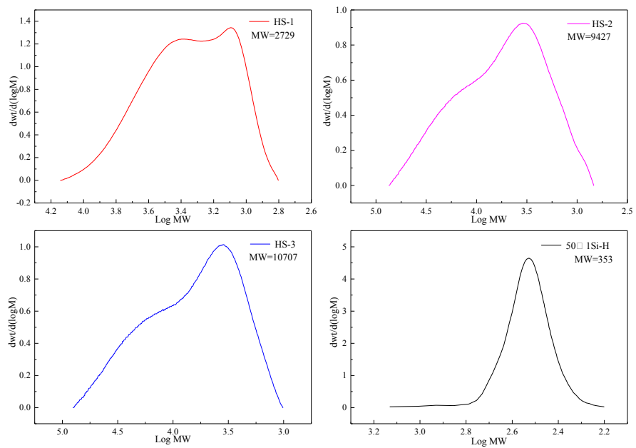
Fig.S1 GPC spectrum of HS series thickener
