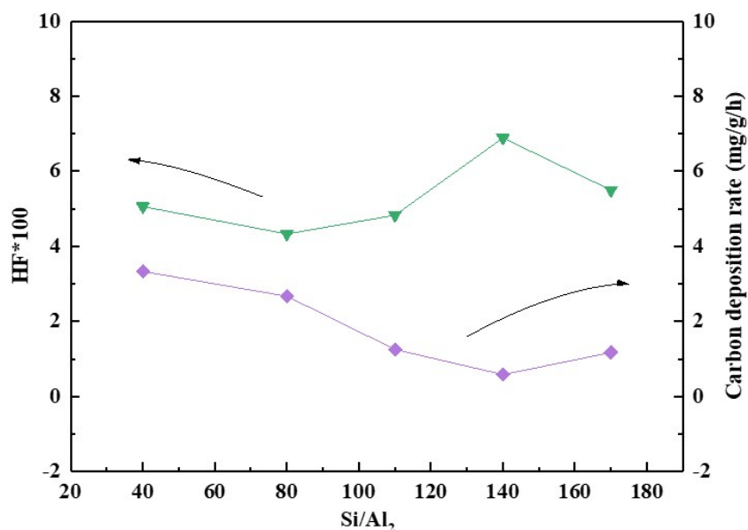
Fig.S1 Variation of HF and carbon deposition rate with \text{Si}/\text{Al}_2 ratio of IM-5 samples
