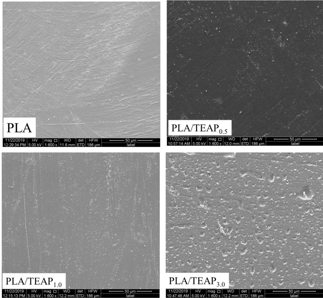
Fig.S1 SEM images for the hot pressed surfaces of samples
