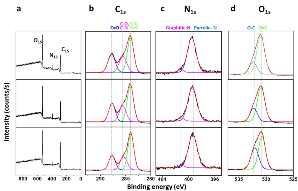
a) XPS survey scan profiles and high-resolution b) C1s, c) N1s, and d) O1s spectra of N-CD 2 from three different batches.
