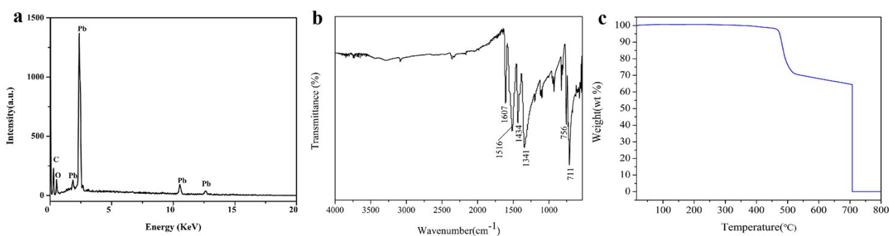
Figure S1. (a) EDS (b) IR spectrum (c) Thermal gravimetric analysis of sample HT.
