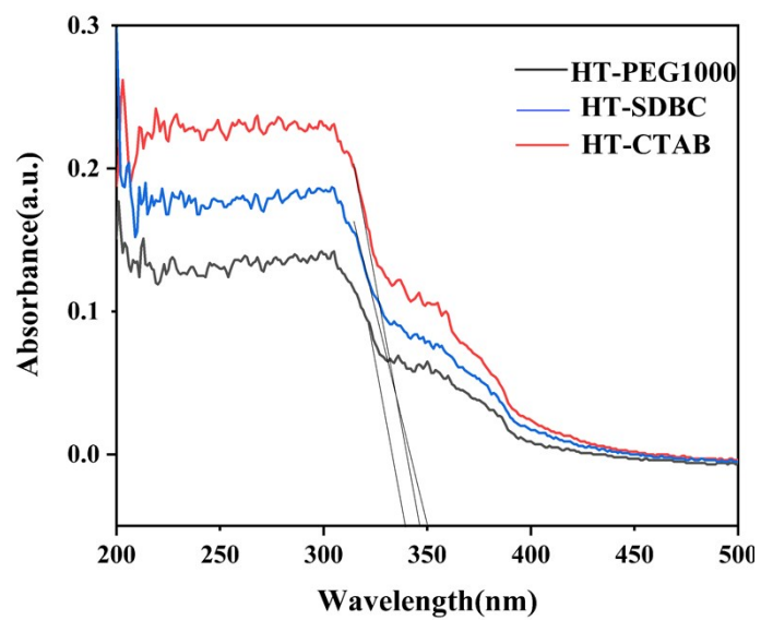
Figure S2. UV - Vis diffuses reflectance spectra of samples prepared by different surfactants.
