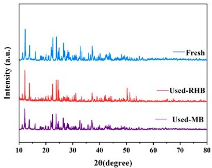
Figure S3. XRD patterns of the fresh and the used HT after 5 recycling runs.
