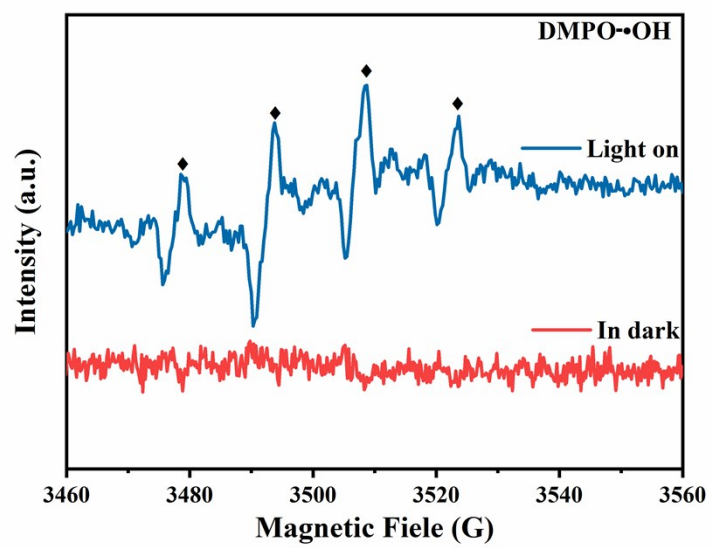
Figure S4. EPR signals of the DMPO-OH with irradiation for 7 min.
