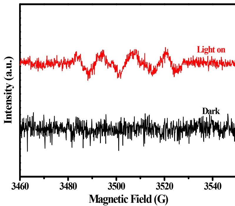
Fig. S2 The ESR spectra of O_2\cdot^- trapped by DMPO over L4C sample dispersion under darkness and light irradiation.
