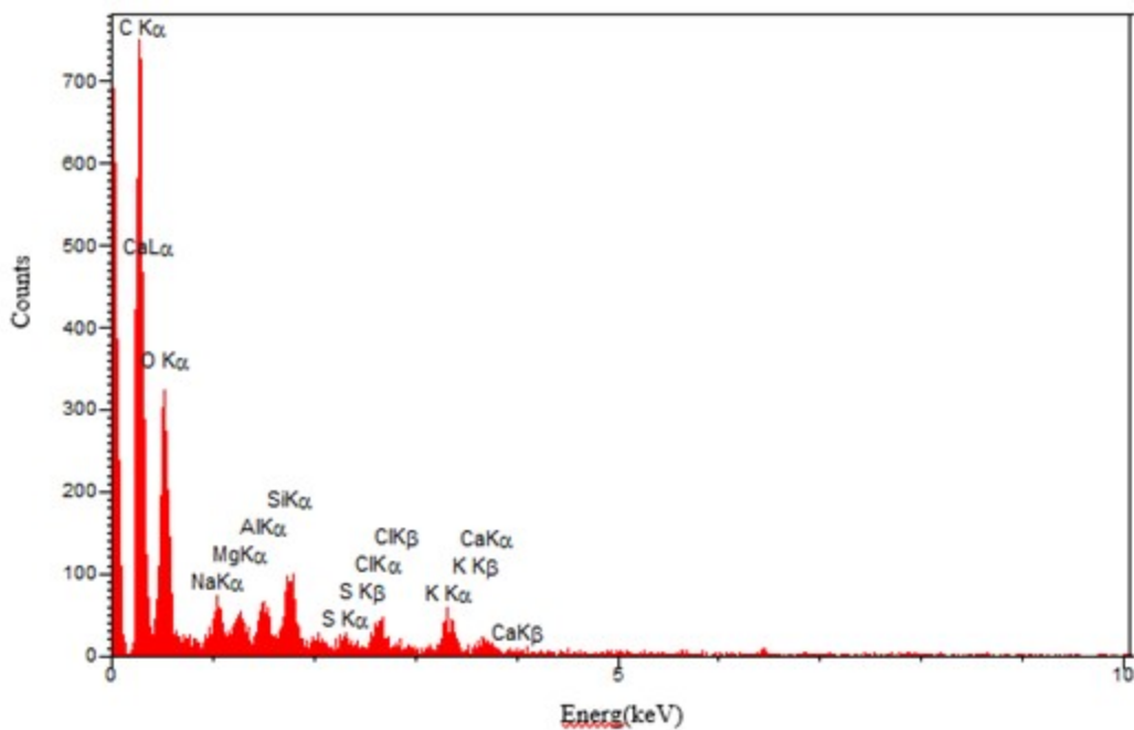
Fig. S1. EDAX spectra of azolla
