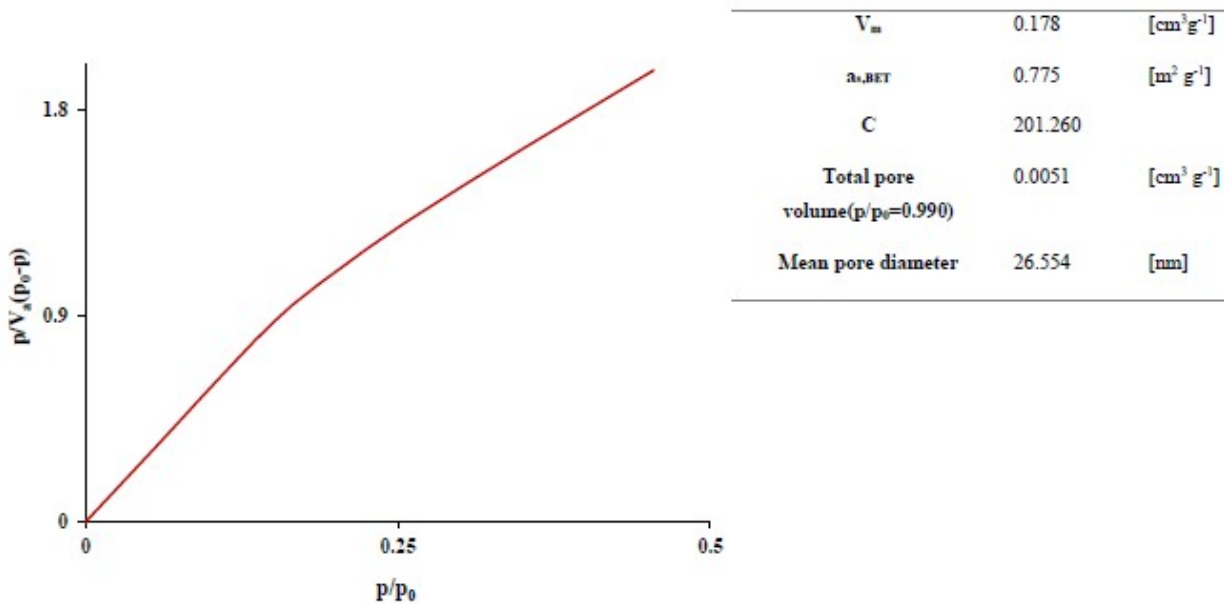
Fig.S2. BET plot of Azolla
