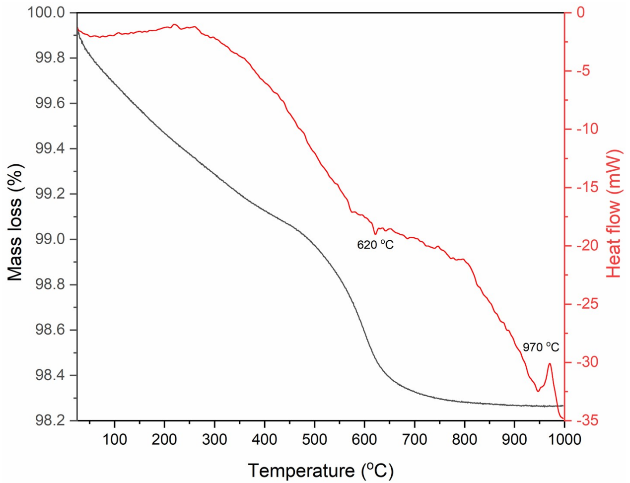
Figure S3. TGA-DSC curves of metakaolin
