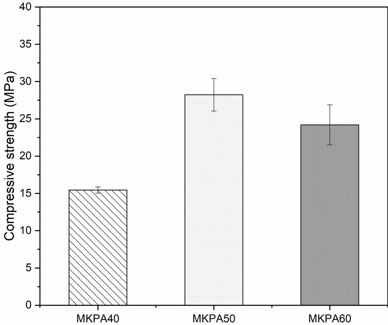
Figure S2. 28-days compressive strength of MK-phosphate geopolymer binder obtain with different concentrations of phosphoric acid (40 wt.%, 50wt.%, and 60wt.%).
