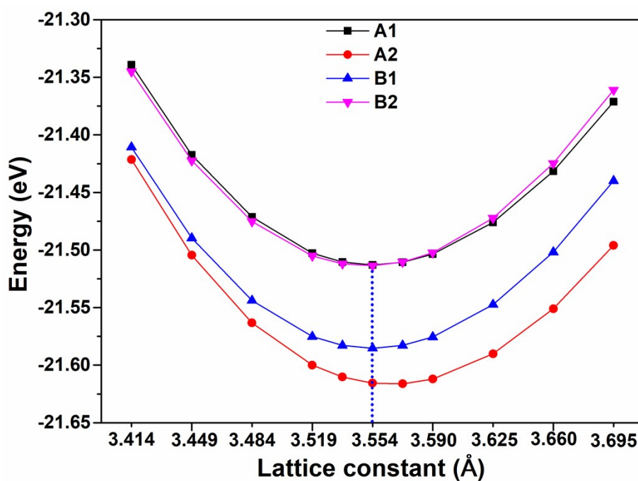
Figure S1. The energy as a function of lattice constant of MoTe 2 /GeS heterojunction.
