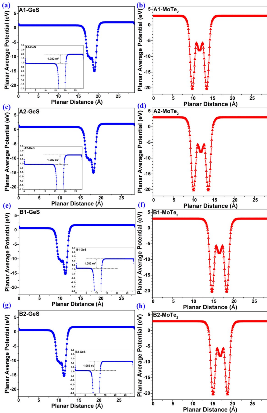
Figure S2. The planar average potential of isolated monolayer GeS and isolated monolayer MoTe 2 for (a,b) A1-, (c,d) A2-, (e,f) B1- and (g,h) B2- stacking structures of MoTe 2 /GeS heterojunction.
