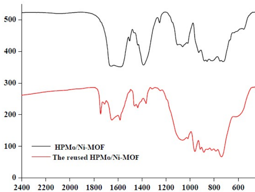
Figure S1. FTIR spectra of the fresh HPMo/Ni-MOF catalyst and used after the tenth runs.
