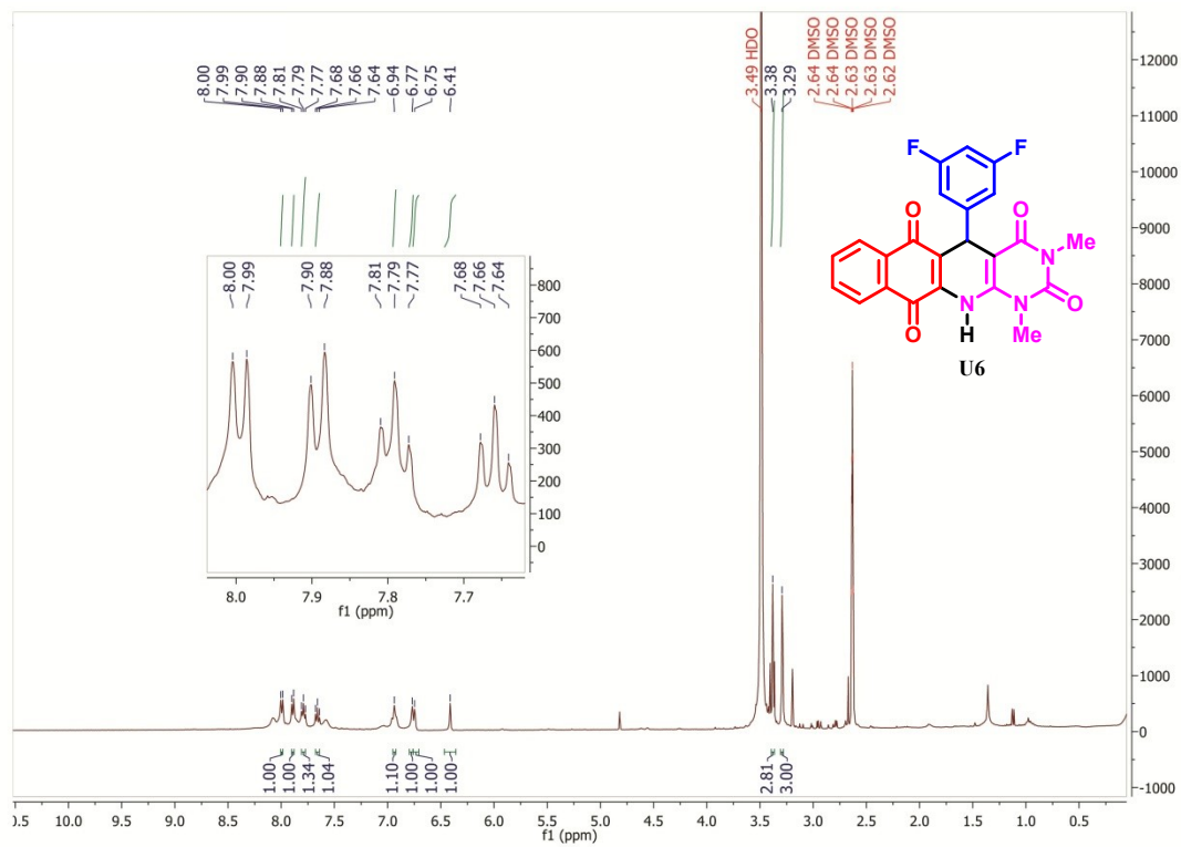
1 H NMR spectrum of 5-(3,5-difluorophenyl)-1,3-dimethyl-5,12-dihydrobenzo[g]pyrimido[4,5-b]quinoline-2,4,6,11(1 H ,3 H )-tetraone (U6).
