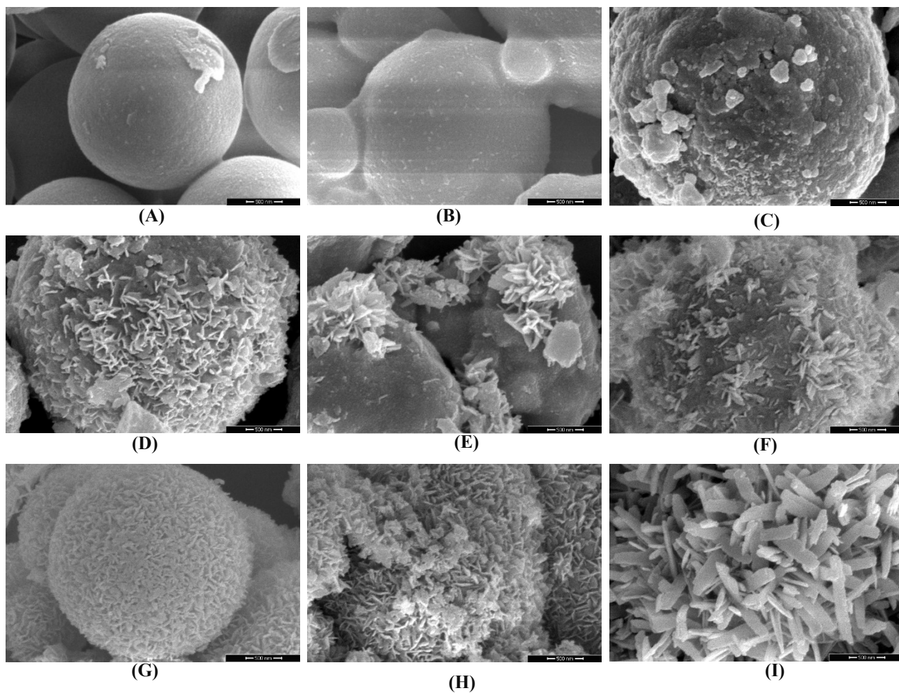
Figure S1 FESEM images (at 2x magnification) of structural characterization of obtained particles at the different conditions of synthesis A (Run 6), B (Run 3), C (Run 1), D (Run 7), E (Run 19), F (Run 4), G (Run 14), H (Run 15), I (Run 5)
