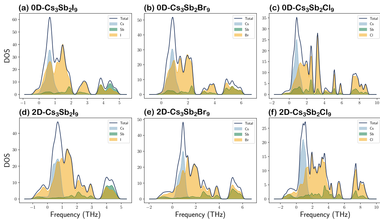
FIG. S1: Total and atom-resolved harmonic phonon density-of-states for 0D and 2D \text{Cs}_3\text{Sb}_2\text{I}_9 .
