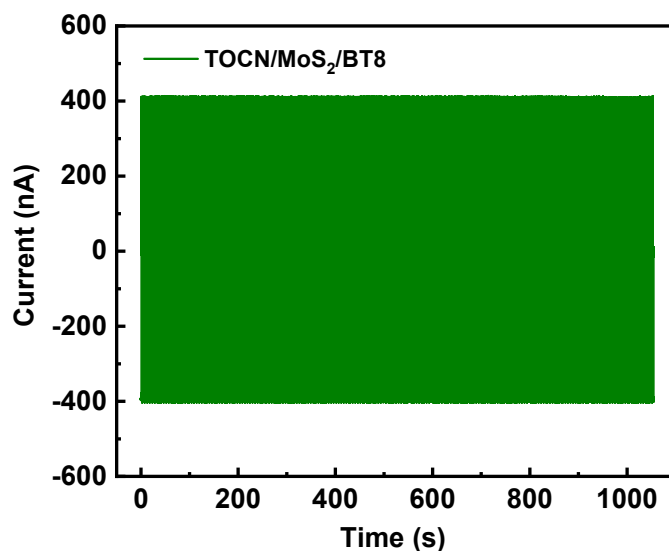
Fig. S1 Durability of short-circuit current for the TOCN/MoS 2 /BT8 composite film-based PENG.
