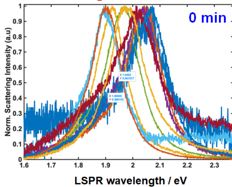
A Before O 2 Plasma Treatment
