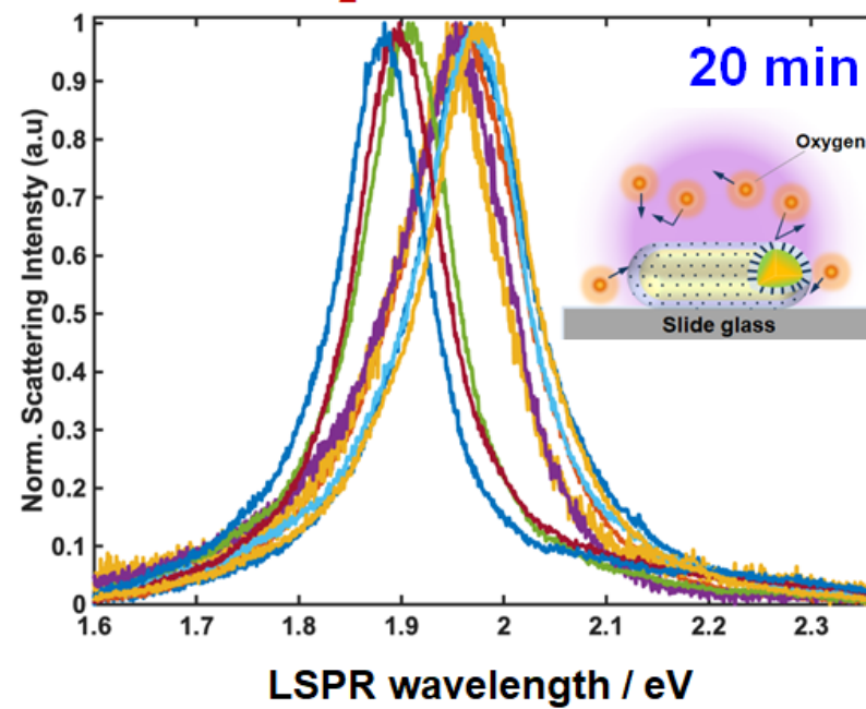
B After O 2 Plasma Treatment
