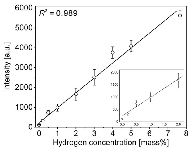
Fig. S1 Calibration curve based on the intensity of the hydrogen emission line (H 656.28 nm line) measured under reduced helium (3000 Pa). (An enlarged calibration curve is shown in the bottom right) Pellets of powder mixtures of Mg and MgH 2 were used as samples 37 .
