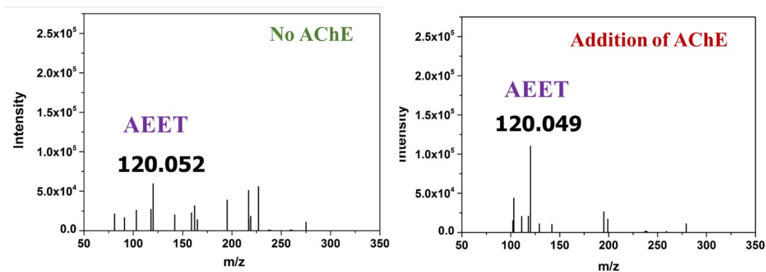
Figure.S2 Monitor of the hydrolysis reaction between AChE and AEET
