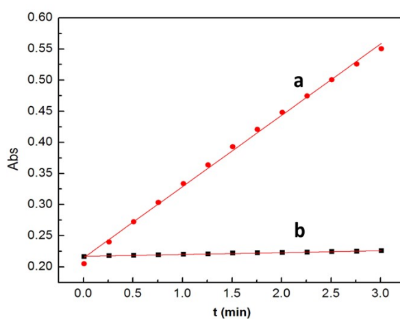
Figure.S3 Enzyme activity assay curve between AChE and ATCh (a) and AEET (b).
