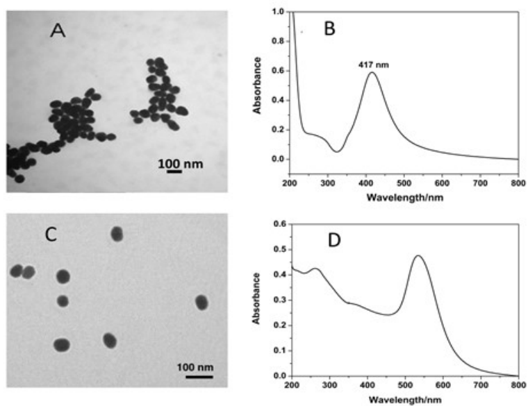
Figure. S1 TEM and UV-Vis of synthesized AgNPs (a,b) and AuNPs (c,d)
