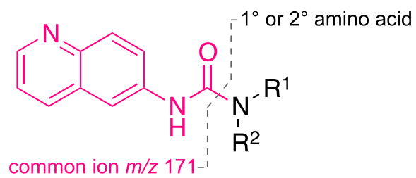
Fig. S1 Fragmentation of 1° and 2° amino acids to produce a common ion ( m/z 171).
