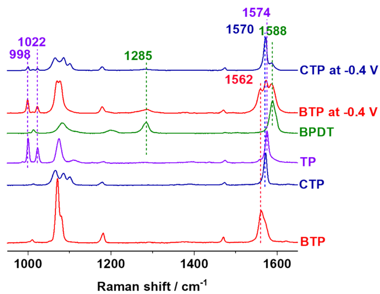
Fig. S1 SHINERS spectra of commercial TP and BPDT on the Ag electrode compared to CTP and BTP at -0.4 V.
