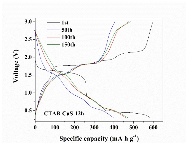
Galvanostatic discharge-charge curves of CTAB-CuS-12h electrode.
