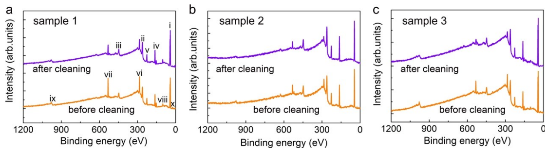
Fig. S2 XPS survey spectra shown from 0 to 1200 eV of the (a) pristine, (b) plasma-treated and (c) plasma-annealing-treated \text{ReS}_2 films before and after the sample cleaning.
