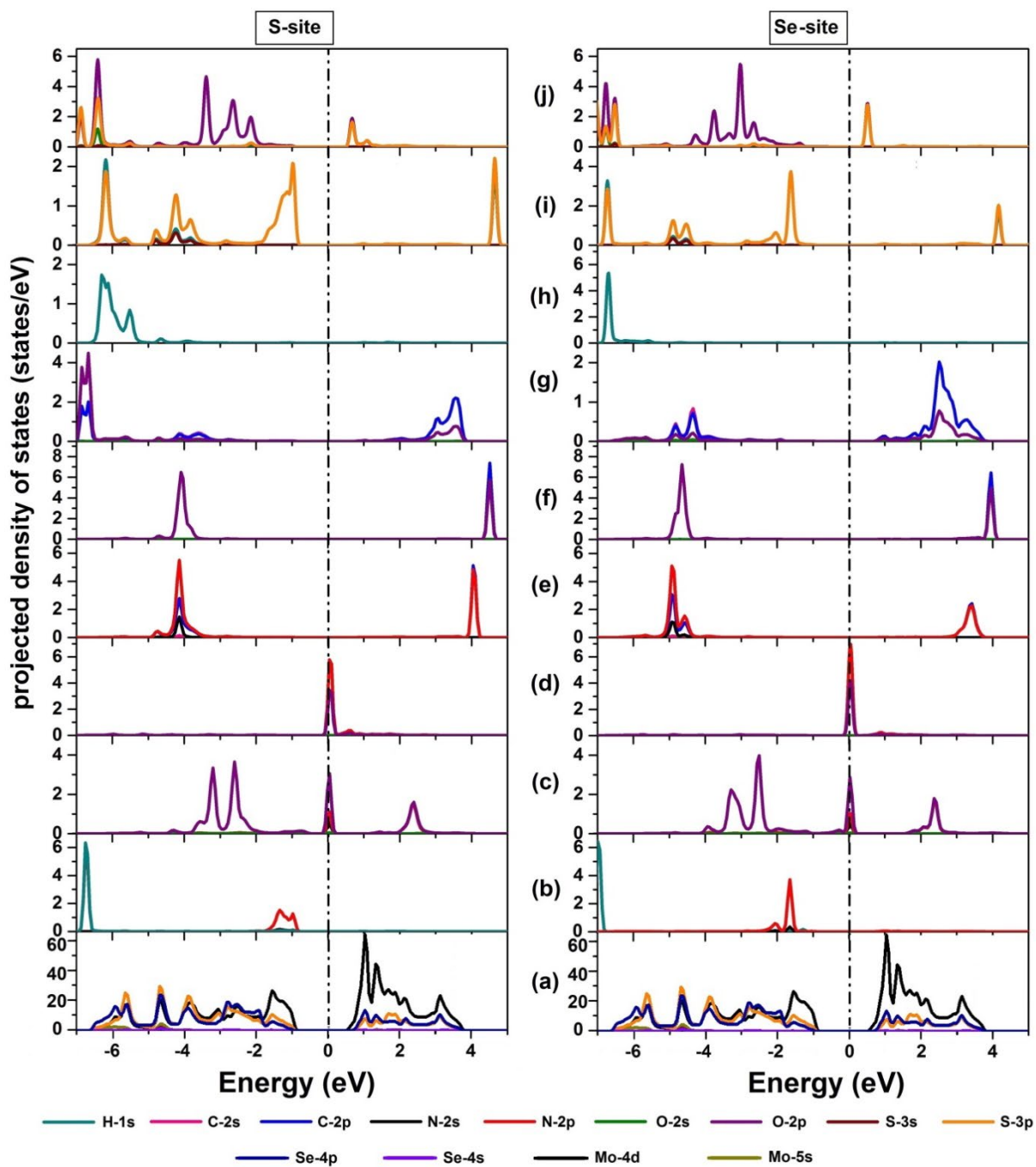
Figure S1. (colour online) PDOS of the adsorbate (a) pristine (b) NH 3 (c) NO 2 (d) NO (e) HCN (f) CO 2 (g) CO (h) H 2 (i) H 2 S and (j) SO 2 on both S and Se site. The dotted line displays the Fermi level set to zero.
