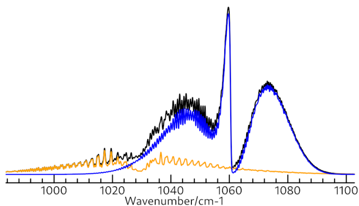
Figure S1 F12-TZ-cCR spectra for \nu_{10} O-C-O antisym stretch (blue), \nu_{11} sym stretch (yellow), and combined (black)
