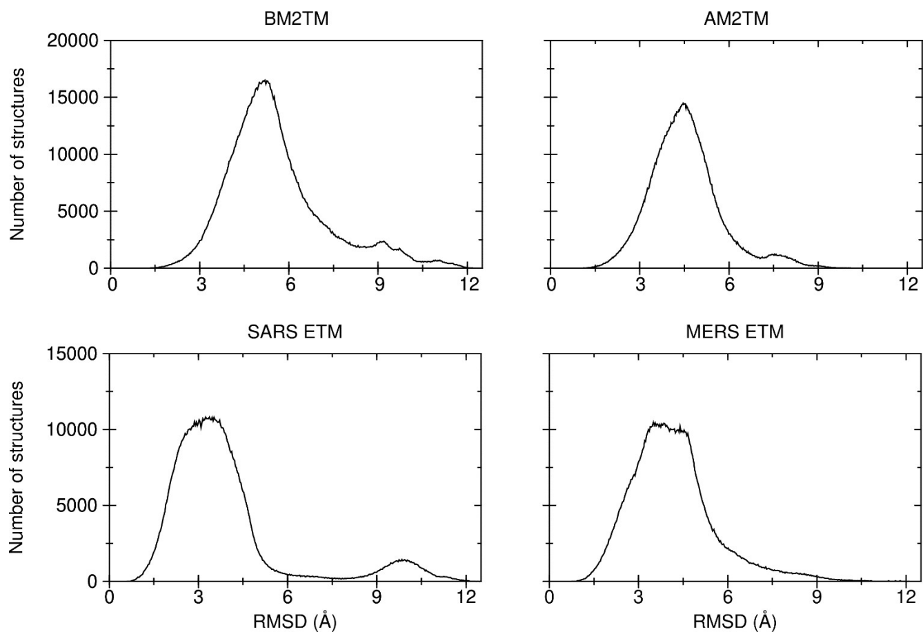
Figure S2. Distribution of the RMSD (Ca carbons) in the calculated snapshots of the peptides tested with folding dynamics.
