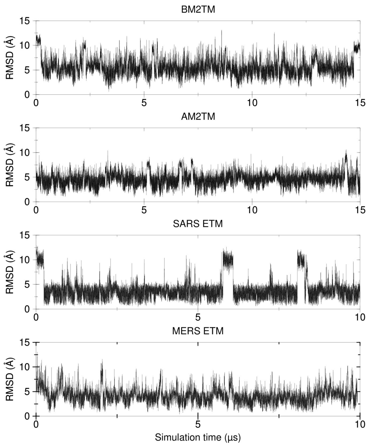
Figure S1. RMSD (Ca carbons) of peptides tested for the 10 μs or 15 μs of folding dynamics.
