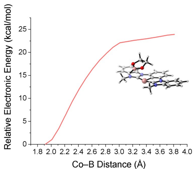
Figure SI2. The potential energy curve for the binding of LCo with Borate
