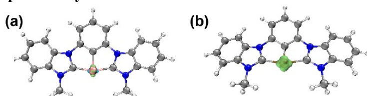
Figure S11. The spin density isosurface of 1LCo (a) and 3LCo (b), at an isovalue of 0.05.
