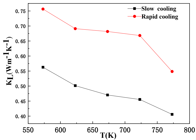
SFig 1 Lattice thermal conductivity of the fast cooling sample and the slow cooling sample in the " \perp " direction
