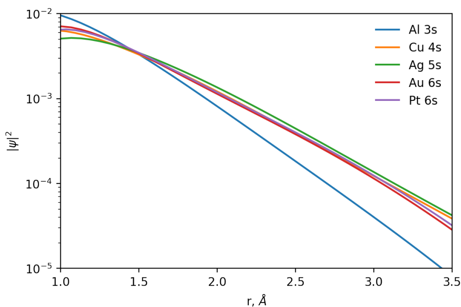
Fig. 1S. Squared single-atom wavefunctions of the Al 3s orbital, Cu 4s orbital, Ag 5s orbital, Au and Pt 6s orbitals obtained by DFT/B3LYP/LanL2DZ.
