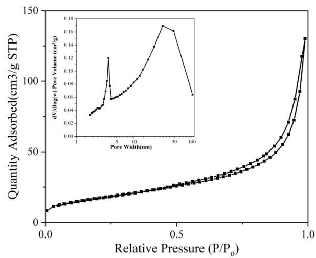
Fig. S3. Nitrogen adsorption and desorption isotherms and pore size distribution (the inset) of bare CNCs.
