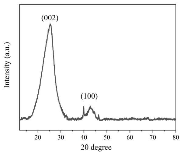
Fig. S2. XRD pattern of bare CNCs.
