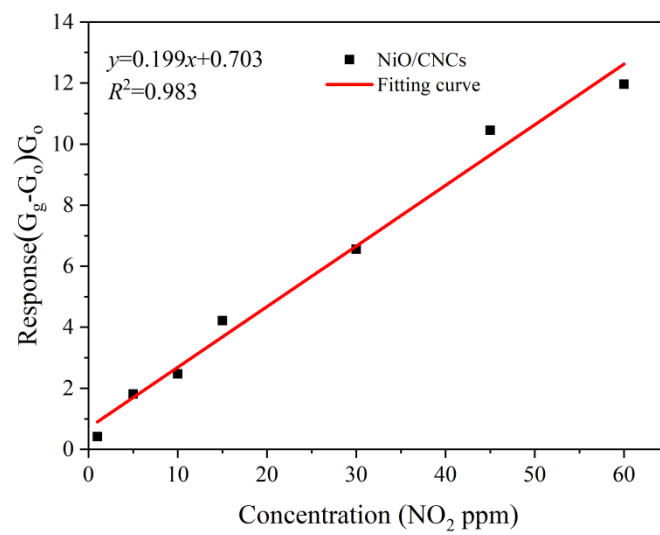
Fig. S4. Fitting curve of 2.0-NiO/CNCs obtained from Fig. 5b.
