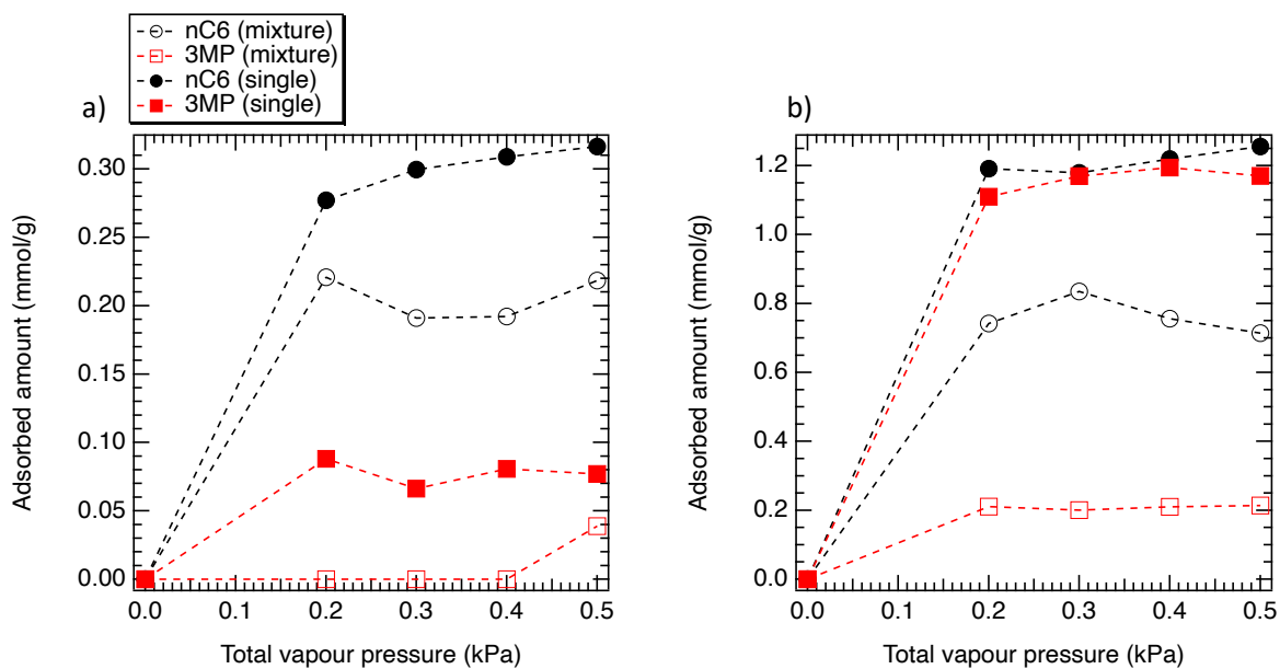
Figure S1: HOMO calculated single and C6/3MP binary component adsorption isotherms of hexane isomers at 343K for a) MIL-140B and b) MIL-140C MOF materials.
