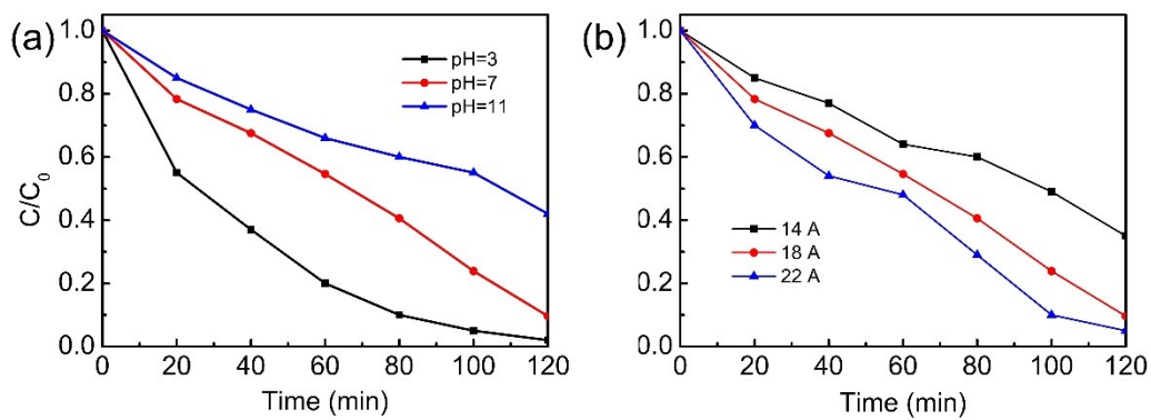
Fig. S6 Degradation of RhB under different pH values (a) and light intensities (b).
