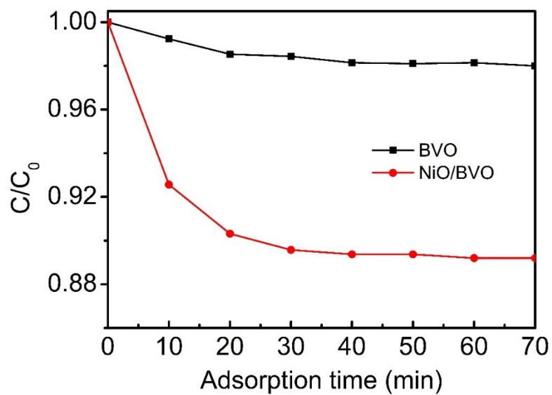
Fig. S5 Adsorption equilibrium curve of BVO and NiO/BVO.
