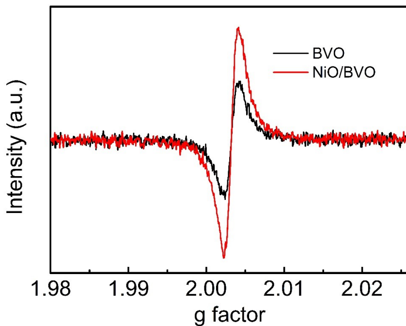
Fig. S3 Low-temperature EPR spectra of BVO and NiO/BVO.
