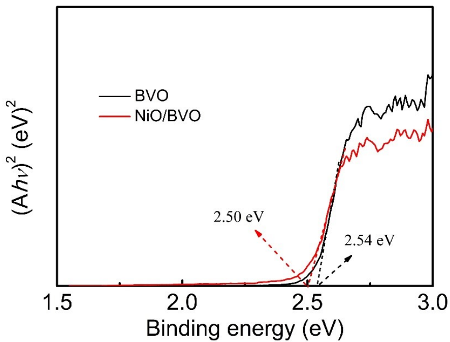
Fig. S4 Optical band gap plots of BVO and NiO/BVO.
