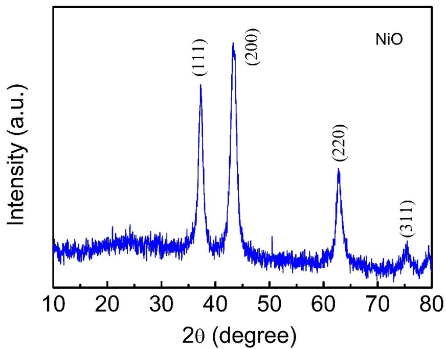
Fig. S1 XRD pattern of NiO.
