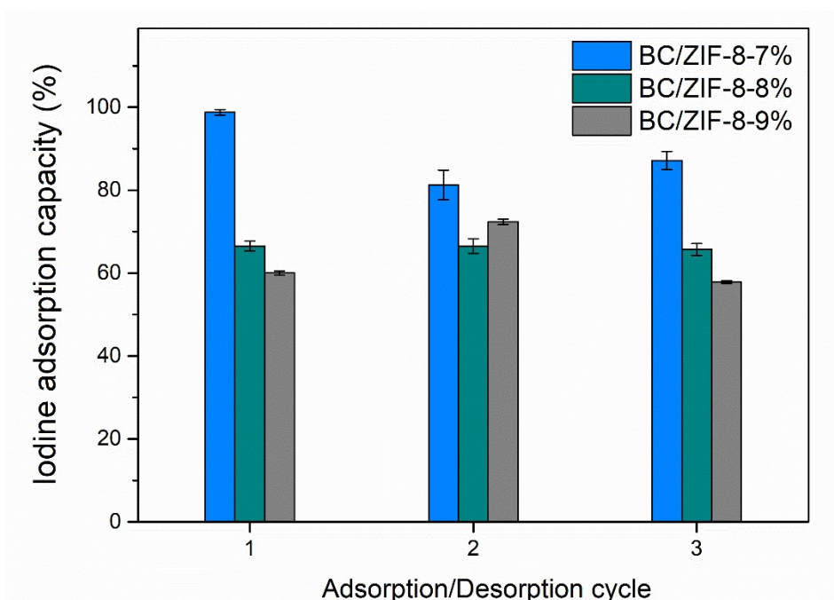
Fig. S1 A recyclability test of BC/ZIF-8 composite
