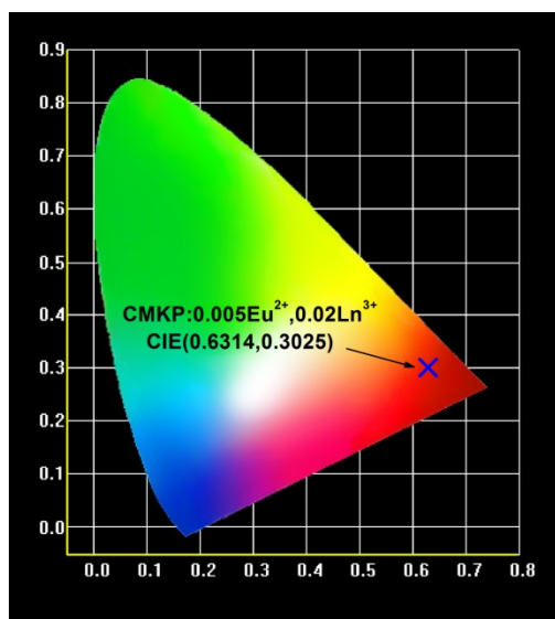
Figure S2. CIE chromaticity diagram corresponding to CMKP:Eu 2+ ,Ln 3+ .
