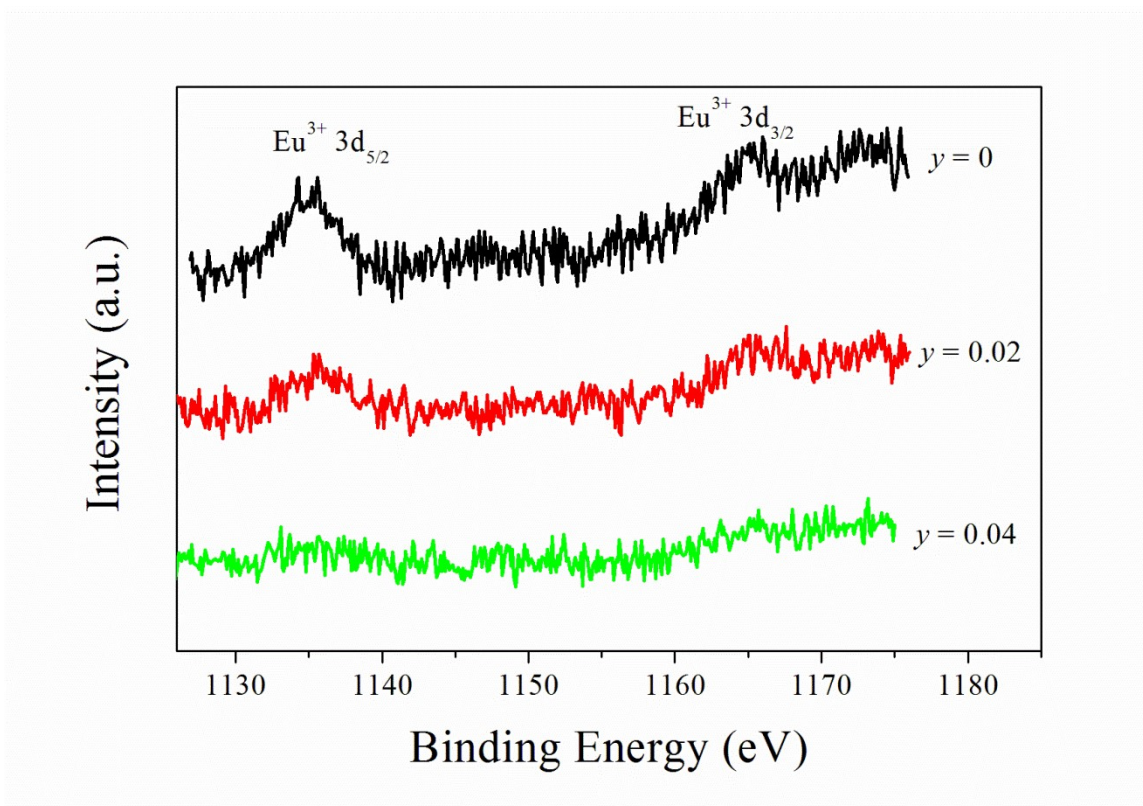
Figure S1. XPS spectra at the Eu 3d 5 position of CMKP:0.005Eu 2+ ,yCe 3+ (y=0, 0.02, 0.04).
