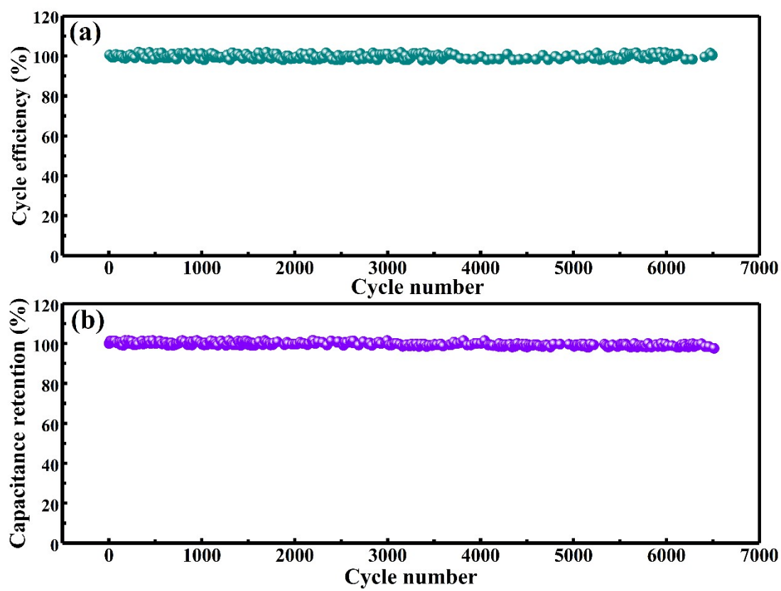
Fig. S1 (a) cycle efficiency and (b) capacitance retention of B-N-P-CSC //B-N-P-CSC-1.
