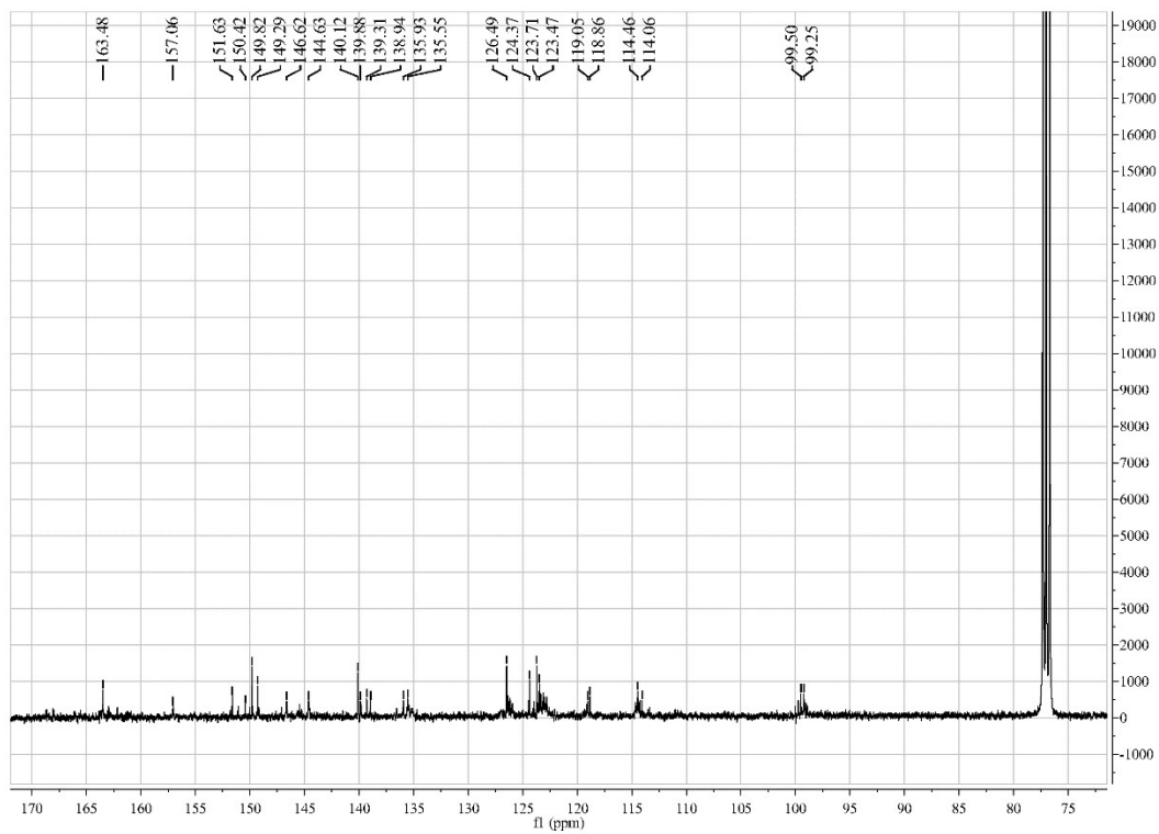
Fig. S8. ^{13}\text{C} NMR spectra of Ir-CF 3 TAZ in \text{CDCl}_3 .
