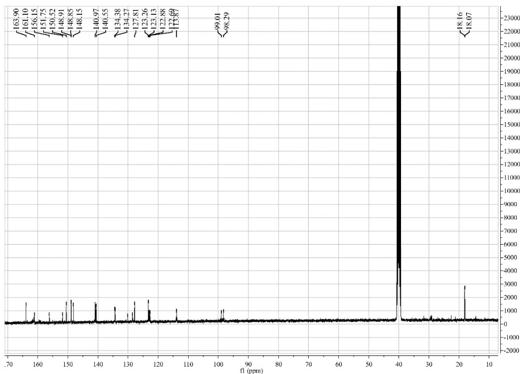
Fig. S2. 13 C NMR spectra of Ir-CH 3 TAZ in DMSO-d 6 .
