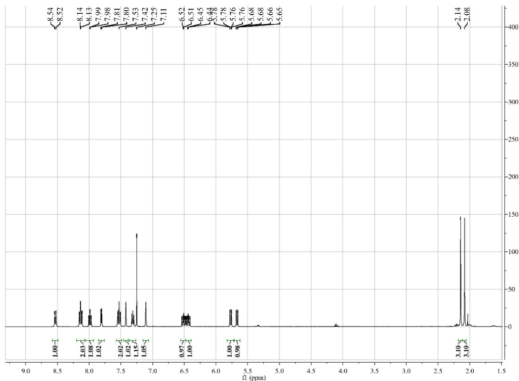
Fig. S1. 1 H NMR spectra of Ir-CH 3 TAZ in CDCl 3 .
