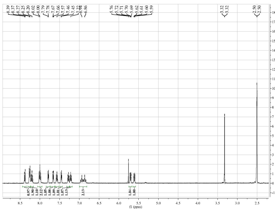
Fig. S4. ^1\text{H} NMR spectra of IrTAZ in DMSO- d_6 .
