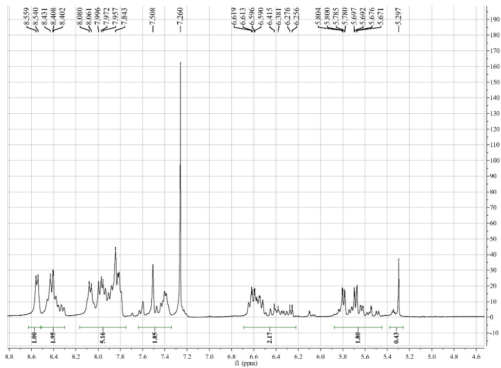
Fig. S7. ^1\text{H} NMR spectra of Ir-CF 3 TAZ in \text{CDCl}_3 .
