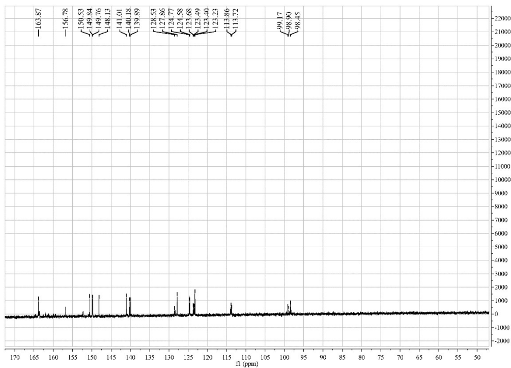
Fig. S5. ^{13}\text{C} NMR spectra of IrTAZ in \text{DMSO-d}_6 .
