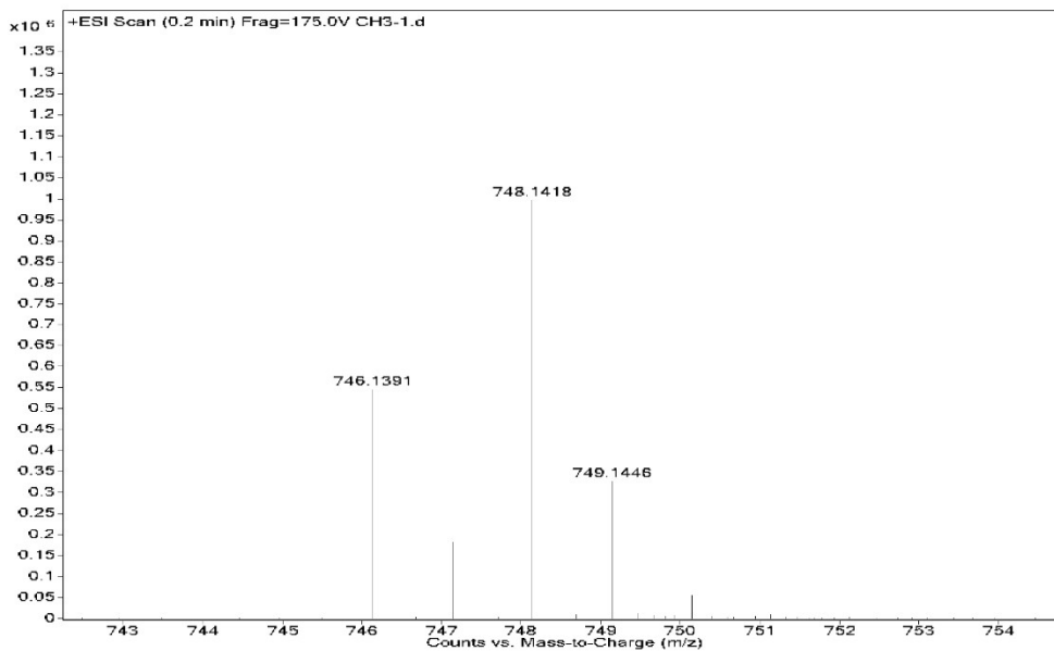
Fig. S3. Mass spectra of Ir-CH3TAZ.
