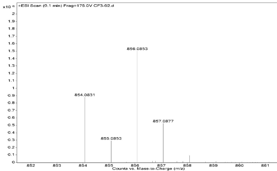
Fig. S9. Mass spectra of Ir-CF 3 TAZ.
