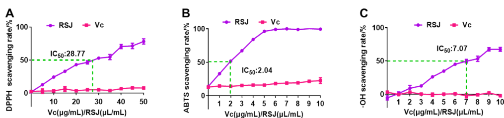
Supplementary Figure S2 The scavenging rate of RSJ on DPPH (A), ABTS (B) and \cdot OH (C) free radicals.
