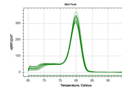
ERK1 Melting curve
