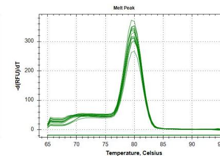
ERK2 Melting curve
