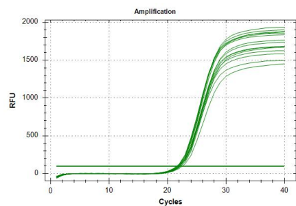
cAMP Amplification plot
