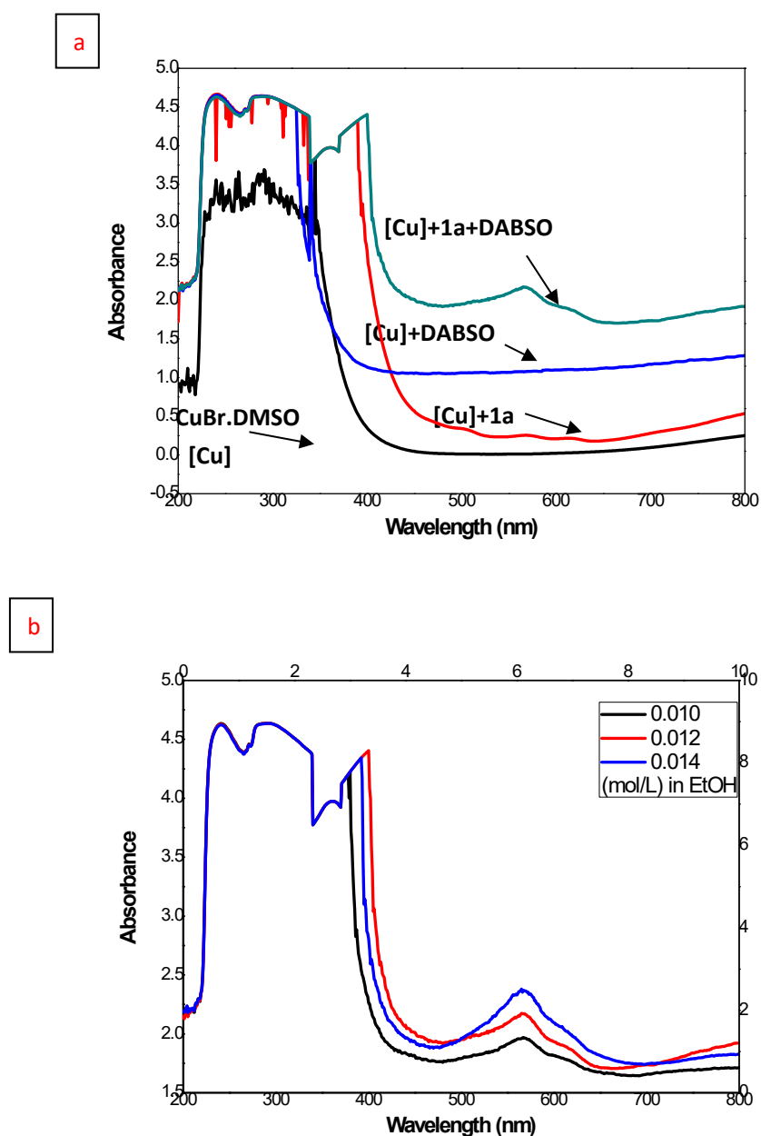
Figure S3: The UV-Visible spectroscopic experiment. (a) CuBr·DMSO (0.01mmol/mL) in EtOH (dark line); both CuBr·DMSO (0.01 mmol/mL) and 1a (0.01 mmol/mL) in EtOH (red line); both CuBr·DMSO (0.01 mmol/mL) and DABSO (0.01 mmol/mL) in EtOH (blue line); CuBr·DMSO (0.01 mmol/mL), 1a (0.01 mmol/mL) and DABSO (0.01 mmol/mL) in EtOH (green line). (b) CuBr·DMSO (0.01 mmol/mL), DABSO (0.01 mmol/mL) and various concentrations of 1a in EtOH.
