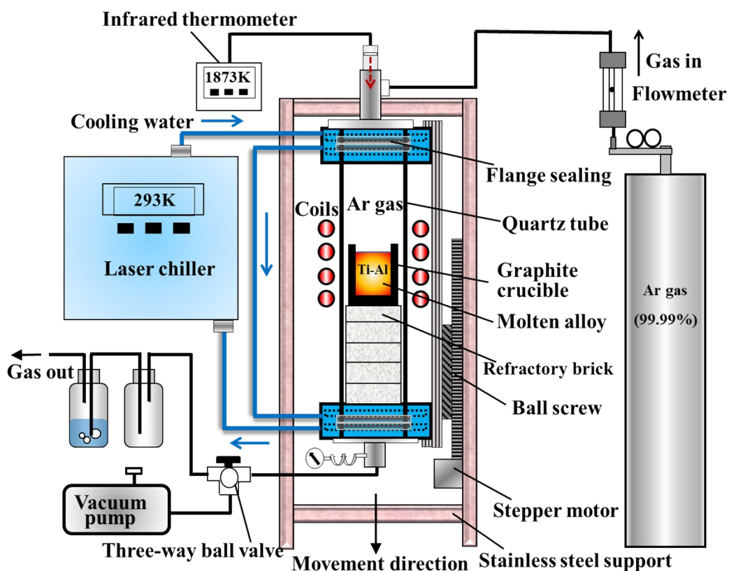
Fig. A.2. Induction furnace with directional crystallization system.
