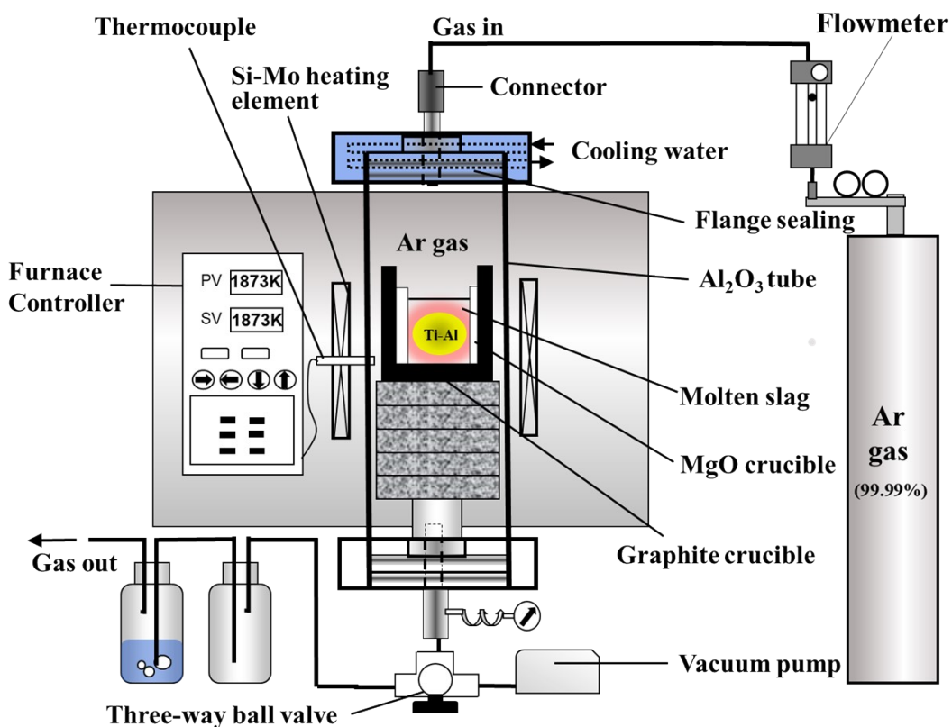
Fig. A.1. Si-Mo resistance furnace.
