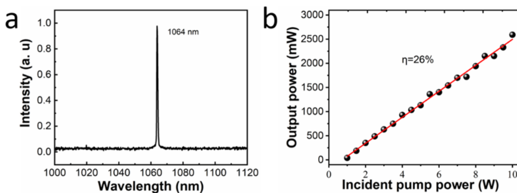
Figure S1. (a) Emission spectrum and (b) conversion efficiency of Q-switched laser without saturable absorber.
