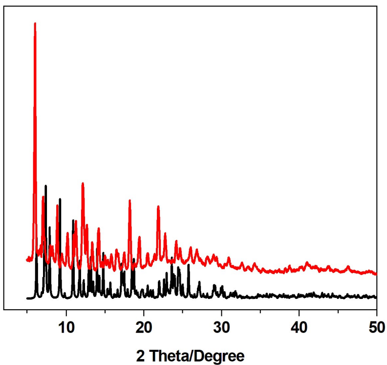
Fig. S8 XRD patterns of simulated Cu-CP (black), as-synthesized Cu-CP (red).
