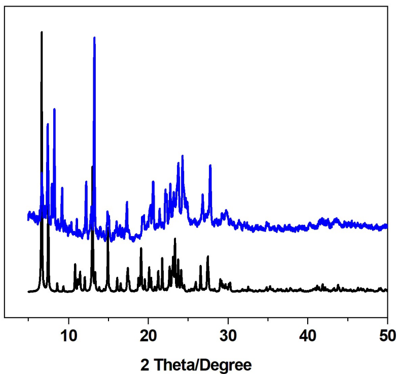
Fig. S7 XRD patterns of simulated Co-CP (black), as-synthesized Co-CP (blue).
