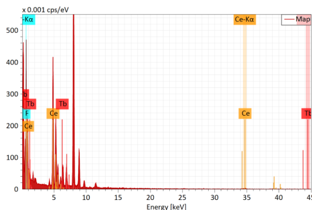
Figure S1. Energy dispersive X-ray (EDX) pattern of \text{CeF}_3:\text{Tb}^{3+} nanoparticles at 1atm.
