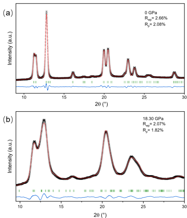
Figure S2. Rietveld analysis result of \text{CeF}_3:\text{Tb}^{3+} nanoparticles before and after structure change, respectively.
