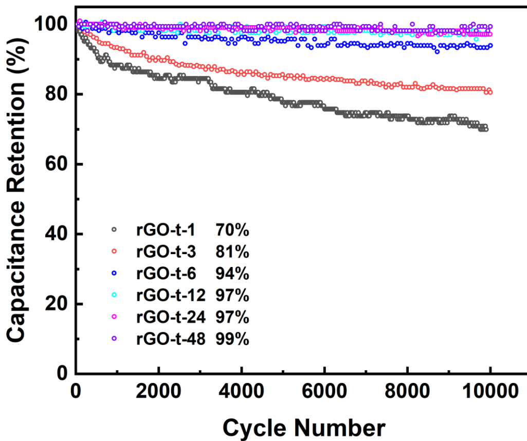
Fig. S5. Cyclic stability of supercapacitors with rGO electrodes.
