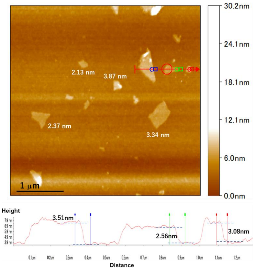
Fig. S2. AFM image (taken in tapping mode) of rGO-t-24 spin-coated onto Si wafer.
