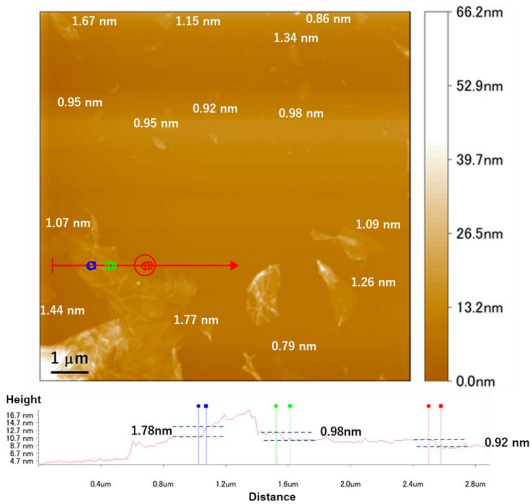
Fig. S1. AFM image (taken in tapping mode) of rGO-t-3 spin-coated onto Si wafer.
