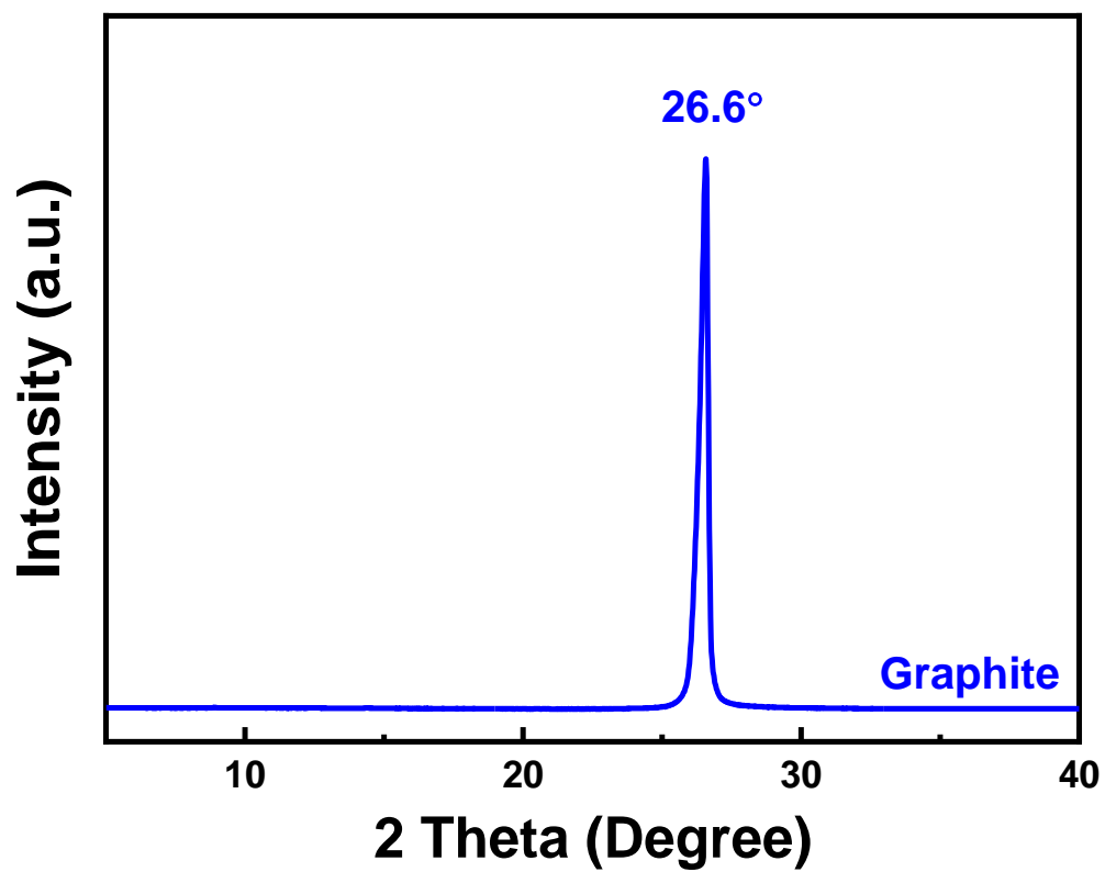
Fig. S3. XRD pattern of graphite powders.
