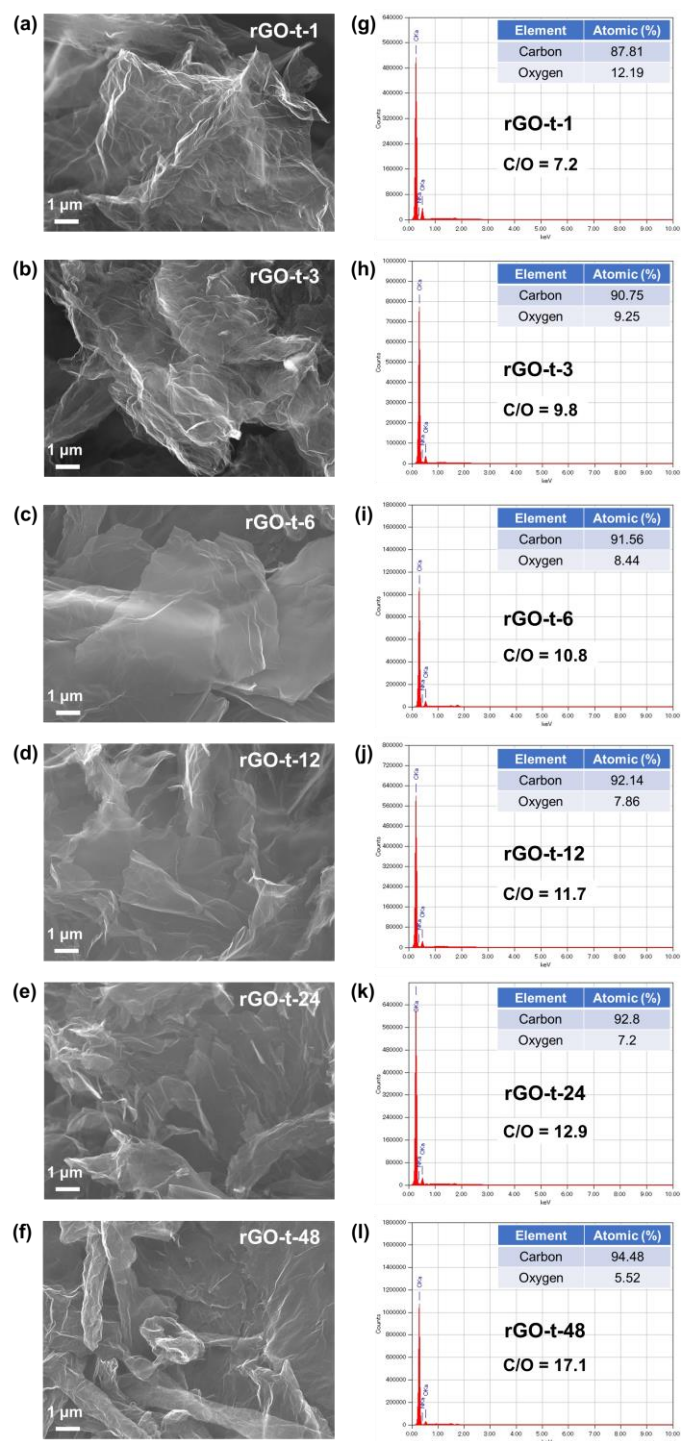
Fig. S4. (a-f) SEM images, (g-l) EDS measurements, and chemical compositions (inset) of rGOs.
