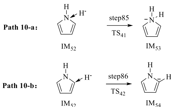
Scheme S2: \text{H}^- attacks the reaction paths of two positions on pyrrole
