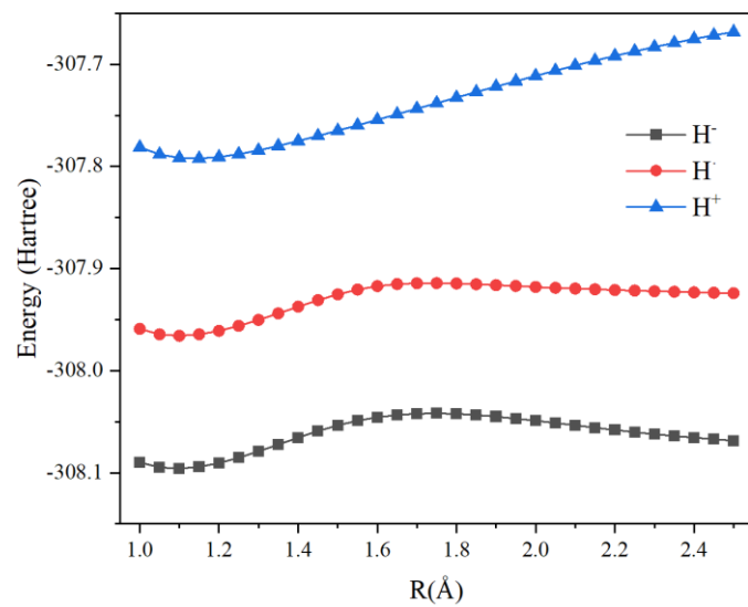
Fig. S1 The scan of the distances between C connected adjacent to O on phenol and H - , H · , and H + (ranged from 1.0 to 2.5 Å, step size 0.05 Å)
