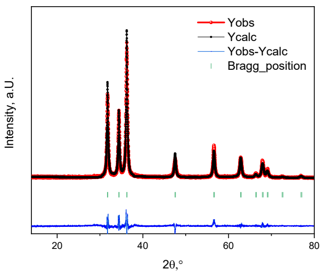
Figure S2: The XRD pattern of an annealed ZIF-8 under Air
