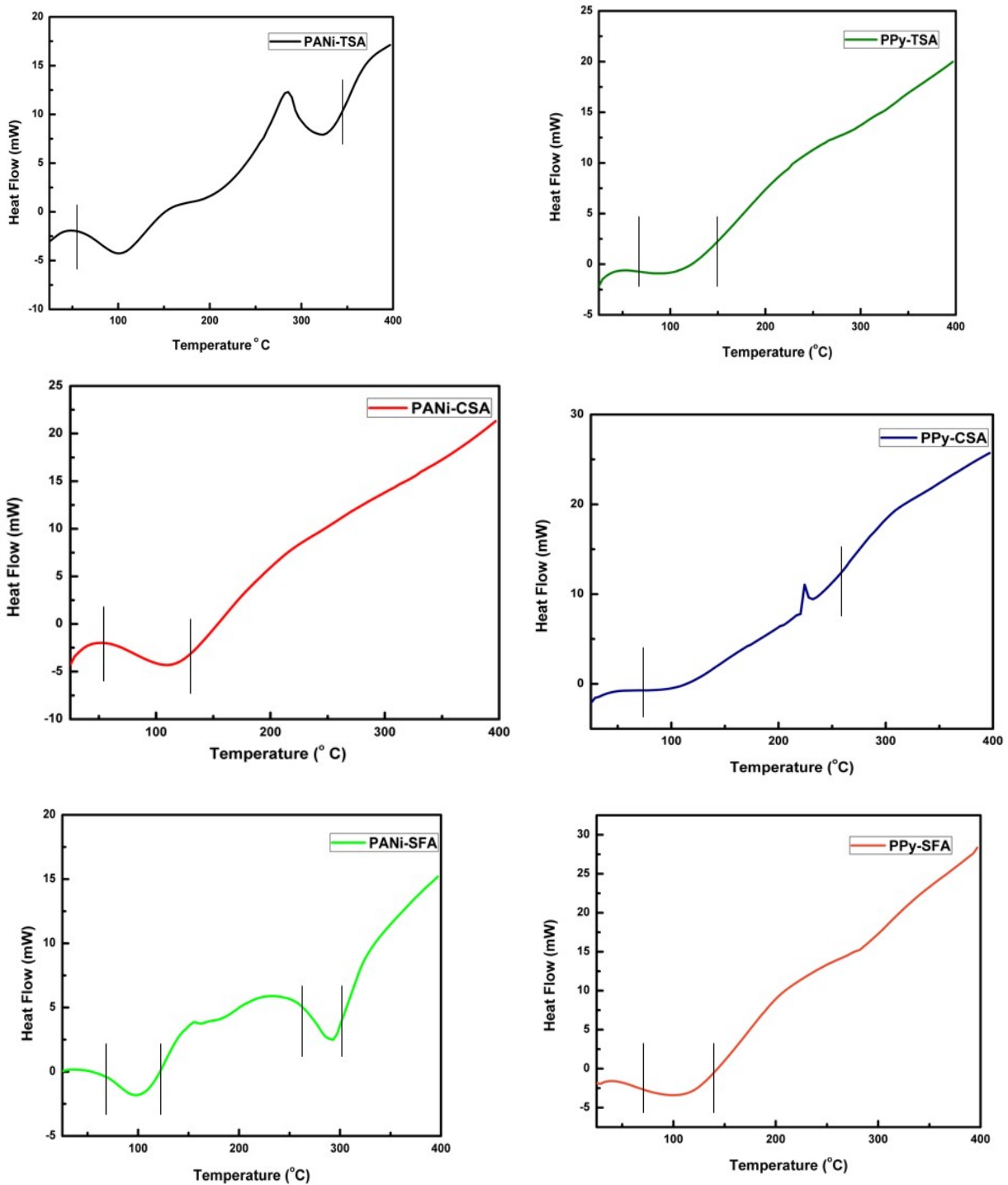
Fig.1S. The DSC curves of sulphonate doped CPs.
