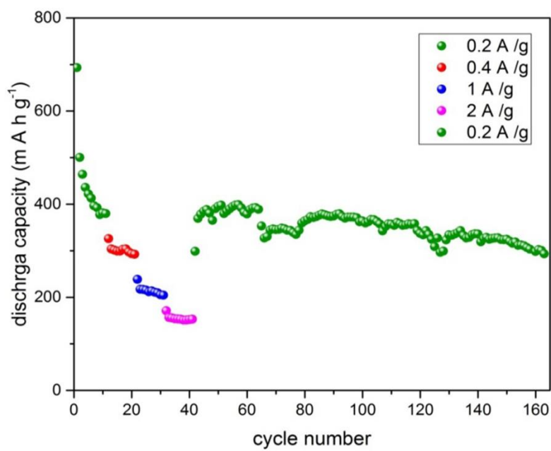
Figure S3. Rateability of TMU-10@CNT with CMC binder
