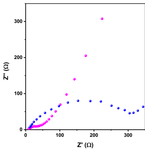
Figure S2. Nyquist plot in high frequency region after cycling
