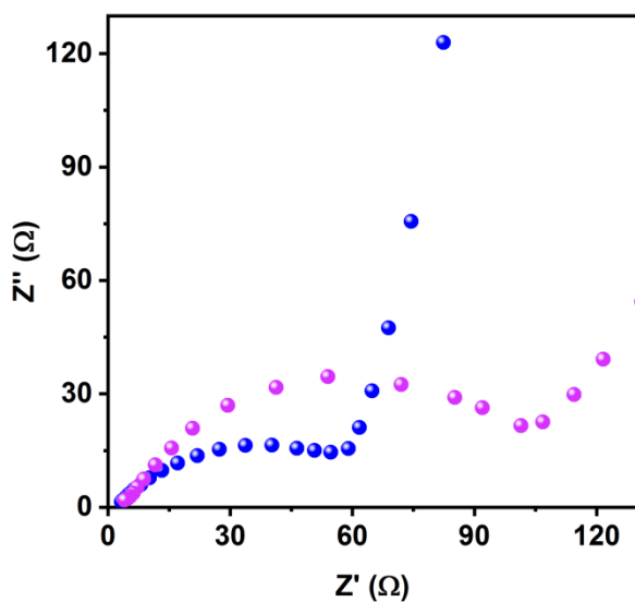
Figure S1. Nyquist plot in high frequency region before cycling
